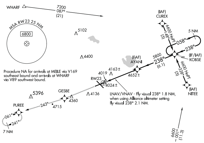
RNAV Approach
